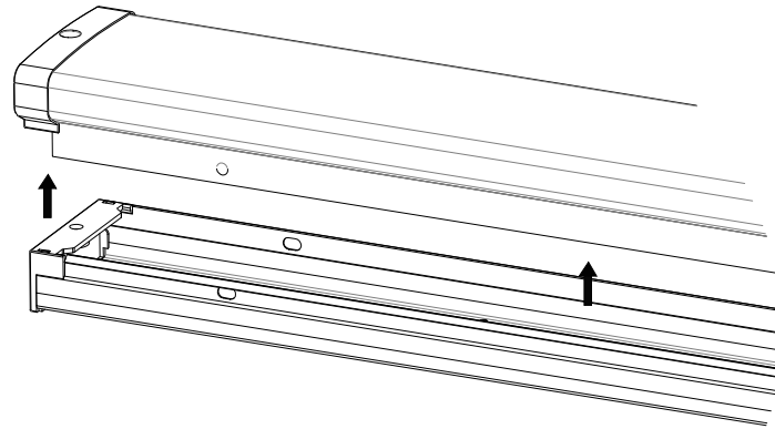
2. Seperate diffuser from housing.
