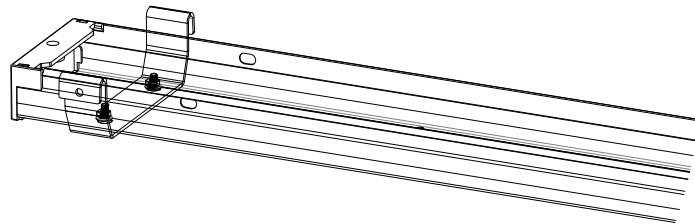
4. Fasten bracket to housing. Repeat on opposing end.
