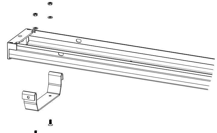
3. Fasten bracket to housing. Repeat on opposite end.
