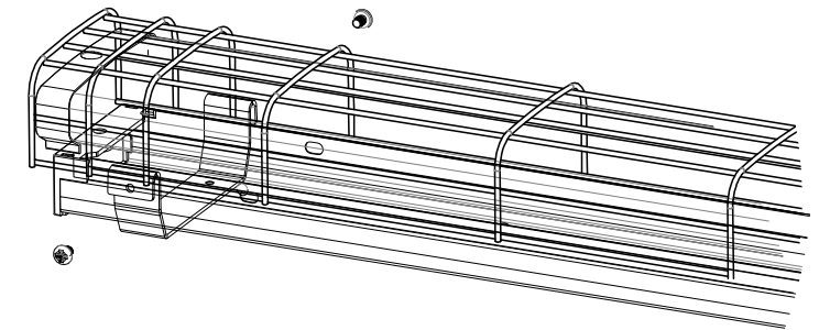
6. Place wire guard into channel of bracket. Secure with screw.
